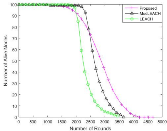
Figure 6. Number of Alive Nodes Comparison
