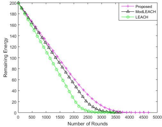
Figure 5. Remaining Energy Comparison
