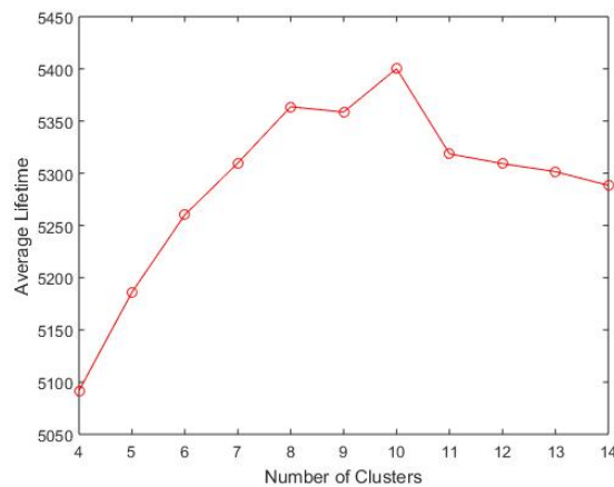
Figure 4. Average Lifetime of the proposed algorithm in terms of varied number of clusters.
